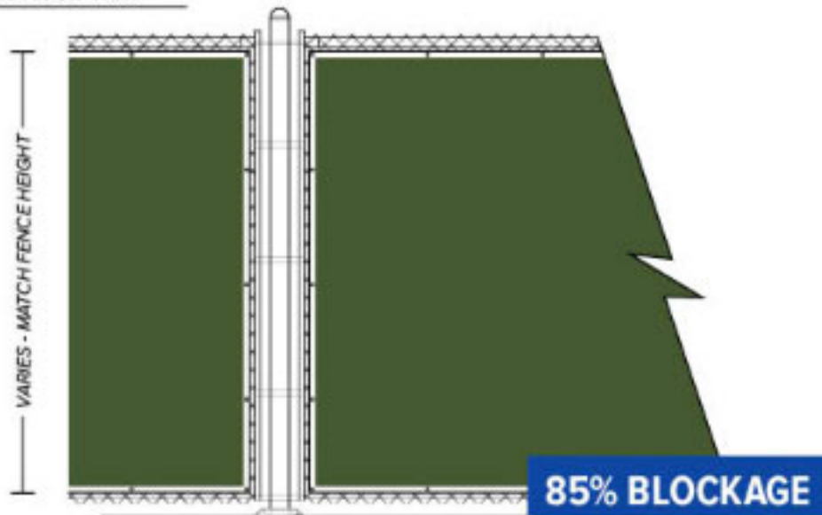
Elevation View
