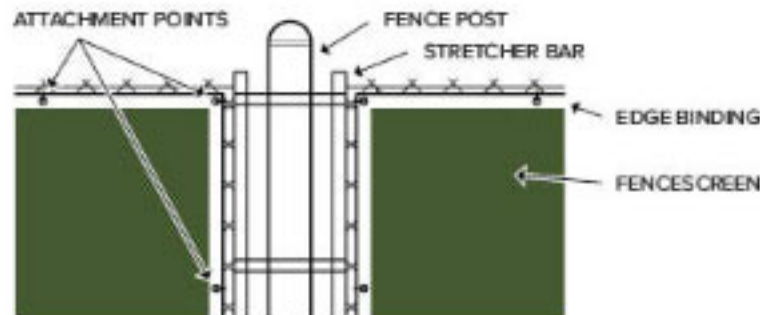
Attachment Enlargement
